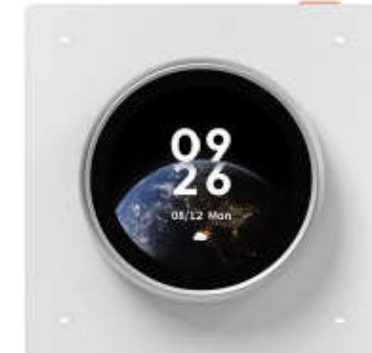
Unit weight: 226g Unit dimensions: 9.5x9.5x7cm Switch Buttons / 3 Built-in Tomato Timer Alarm Smart Knob Control Panel / 1 Knob Control / 2 3-ch Relay & 4-ch Custom CCP-S 03-EU
